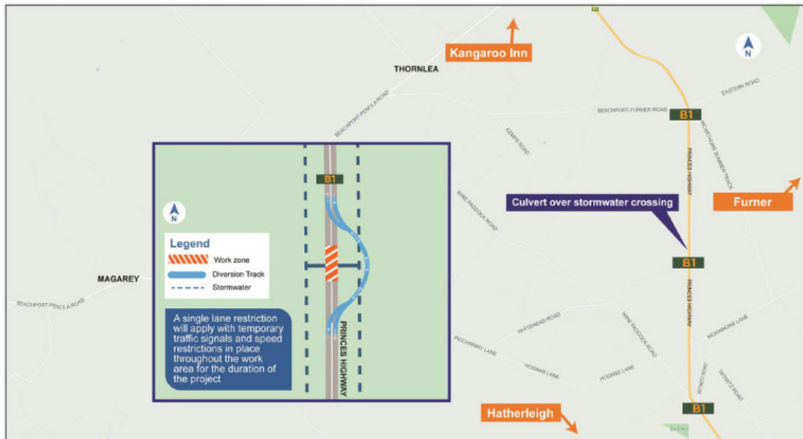
Culvert over stormwater crossing, Princes Highway, Thornlea
