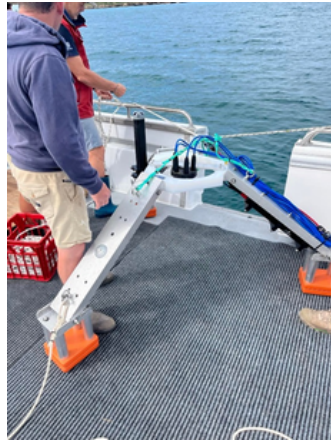
Frame for Monitoring Equipment
